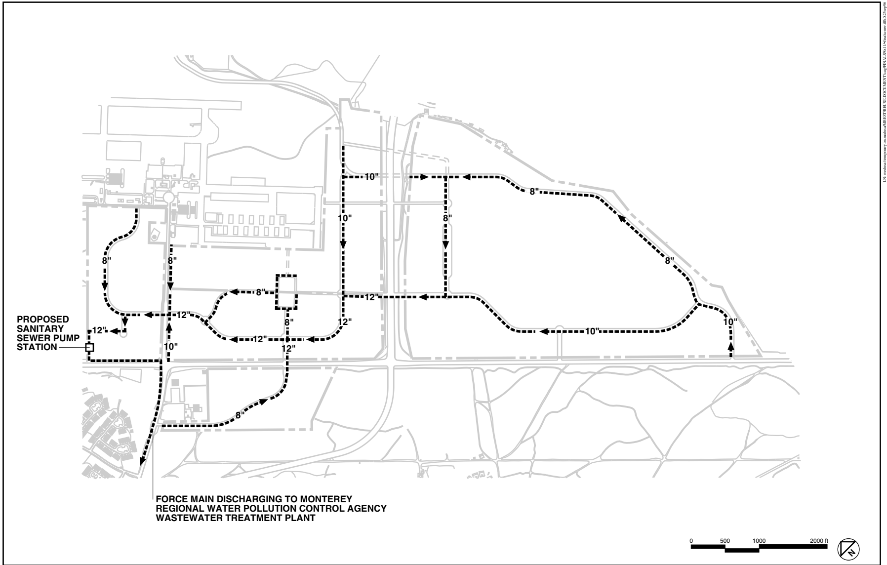
Figure 7.2– Proposed Sanitary Sewer Facilities
